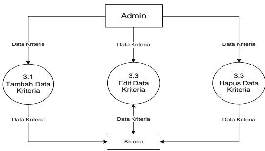
Gambar 3.7 DFD level 1 proses 2 Data Kriteria
