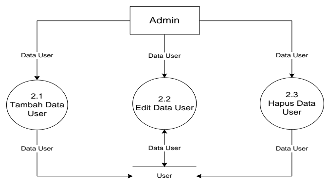
Gambar 3.6 DFD Level 1 proses 1 Data User
