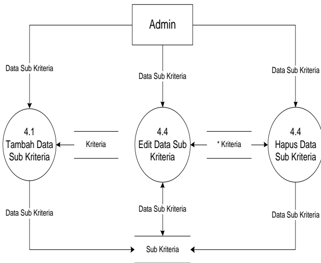
3.8 DFD level 1 proses 3 Data sub kriteria
