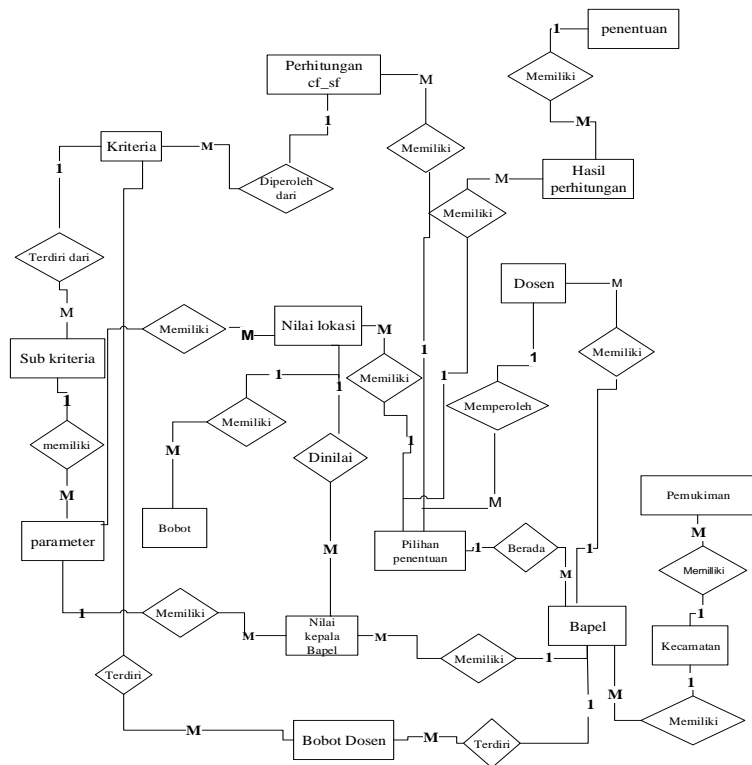
Gambar 3.3 Entity Relationship Diagram SPK Penentuan Dosen Pembimbing Lapangan KKM
