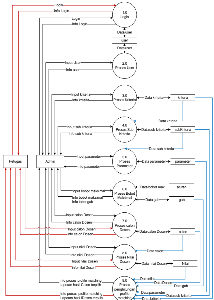
Gambar 3.5 DFD level 0
