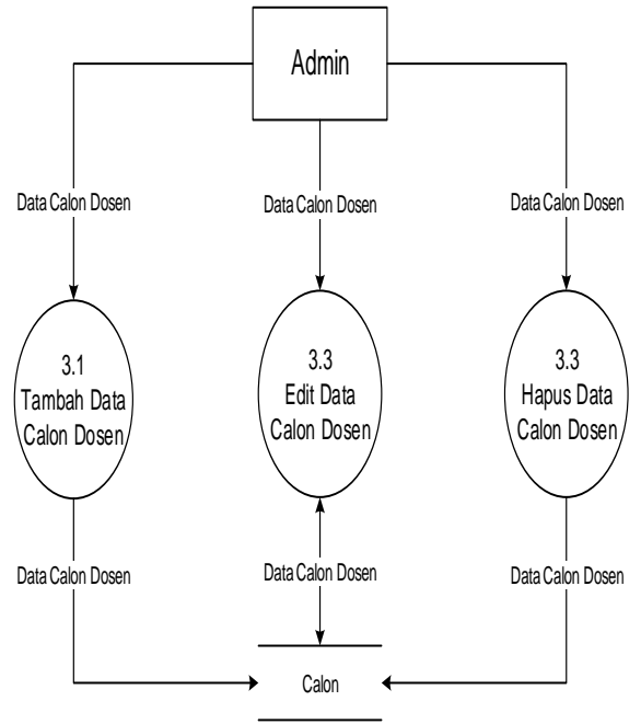
Gambar 3.10 DFD level 1 proses 5 Data Calon
