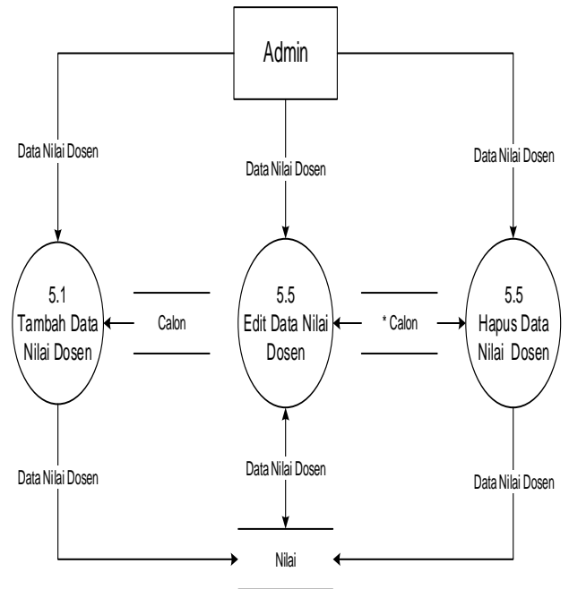
Gambar 3.11 DFD level 1 proses 6 Data Nilai Dosen
